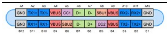
USB Type C pinout
