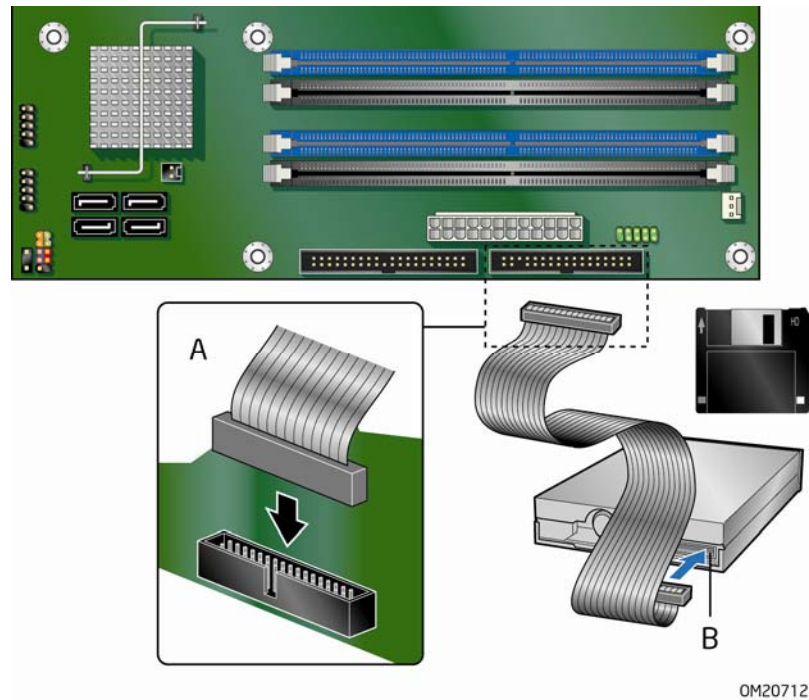
Figure 20. Connecting the Diskette Drive Cable
